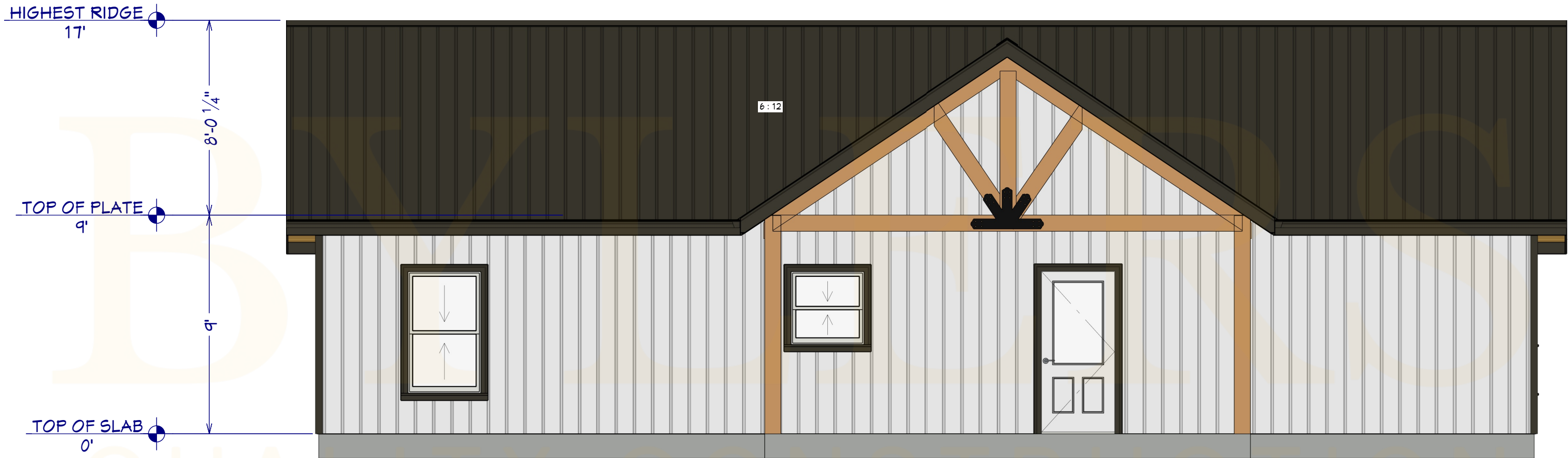
Exterior Elevation Back
